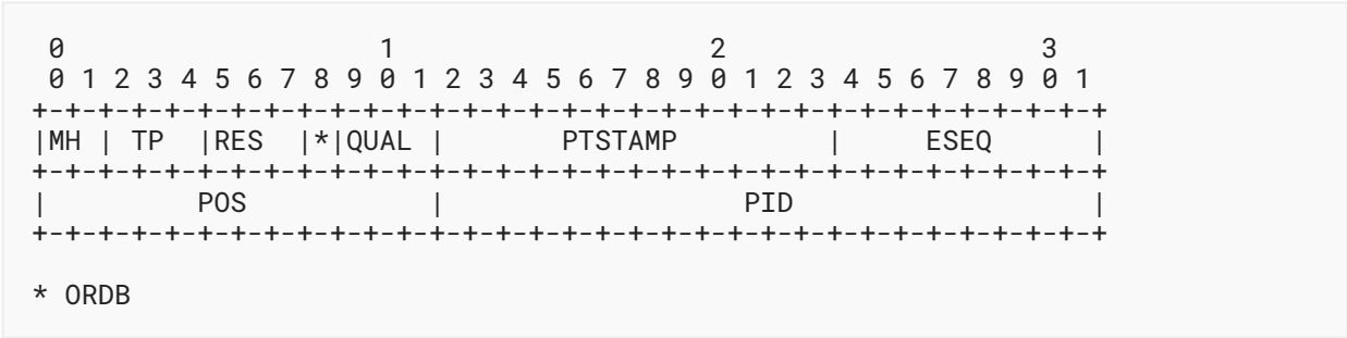
Figure 3: Structure of the Body Packet Payload Header
