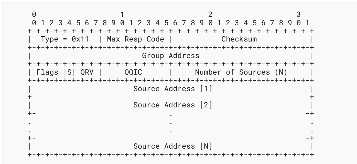
Figure 1: IGMPv3 Query Message
